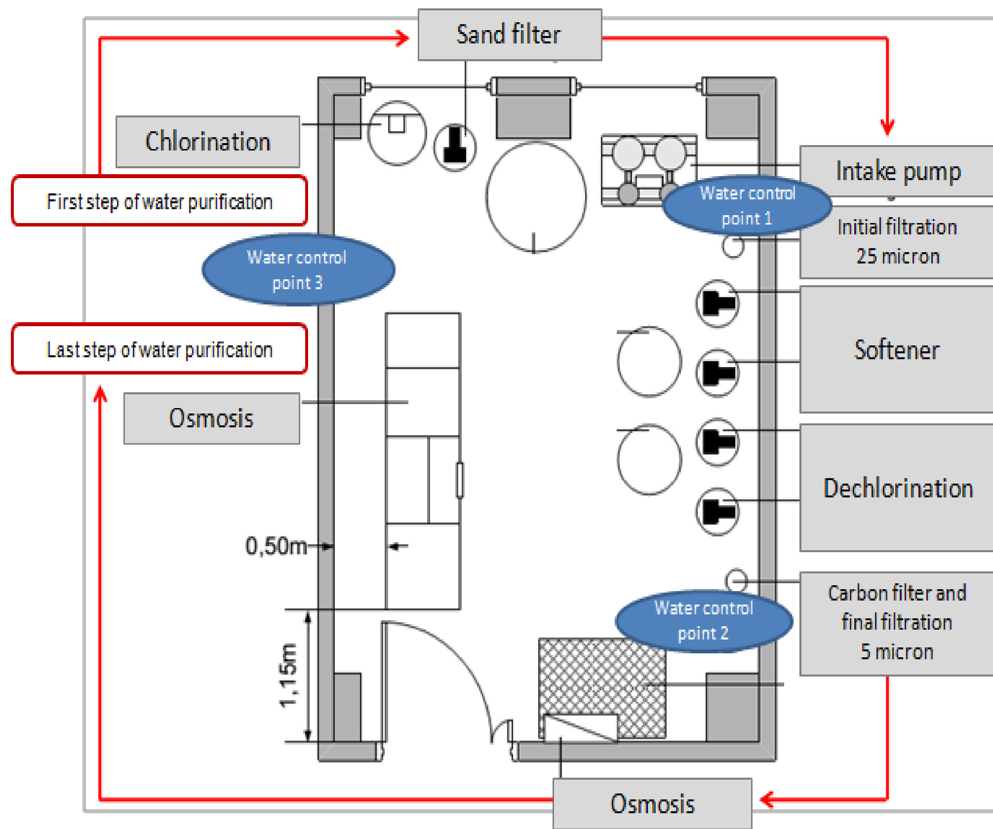
Figure 1. Water purification system used in haemodialysis.
