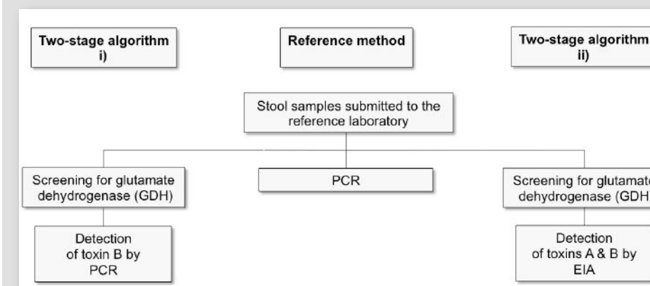
Figure 2: Diagnostic algorithms for C. difficile detection
