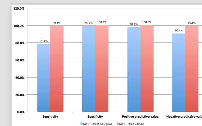
Figure 3: Performance markers of both test algorithms, GDH +Toxin B by PCR in red (i) and GDH+Toxins A+B by EIA in blue (ii)
